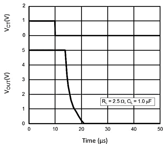
t_{OFF} Response
