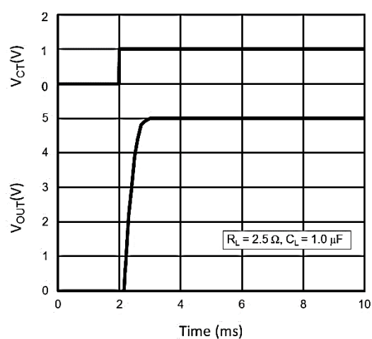
t_{ON} Response
