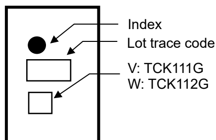
Top Marking
