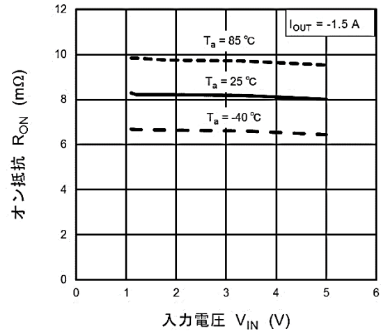
RON - V IN
