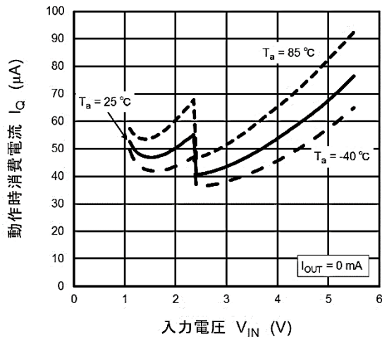
I Q - V IN
