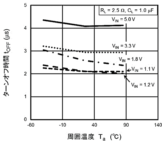
t OFF - T a
