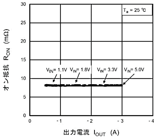
RON - I OUT
