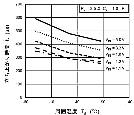
t r - T a
