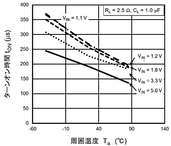
t ON - T a
