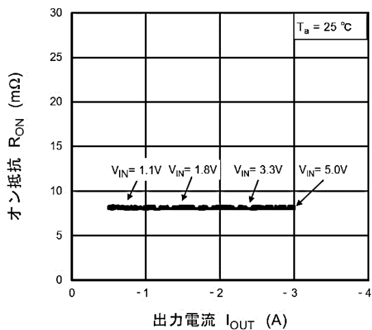
R_{ON} - I_{OUT}
