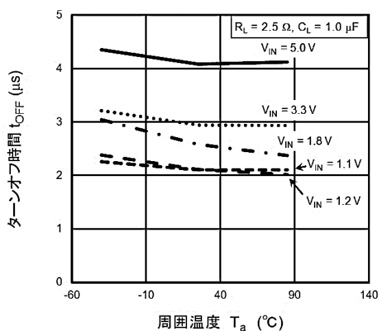
t_{OFF} - T_a
