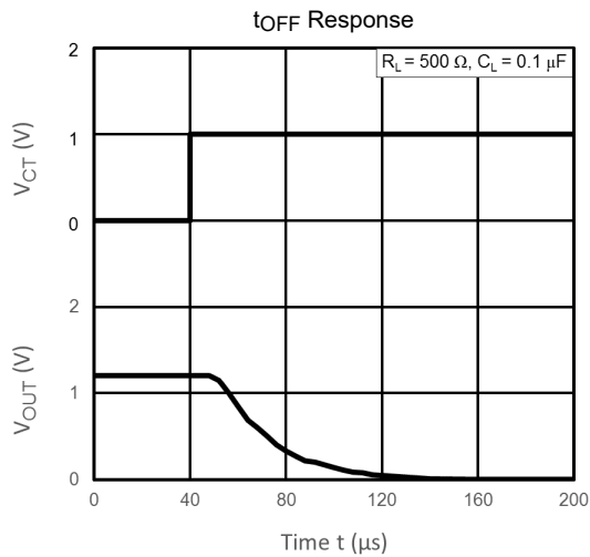
TCK208G Typical characteristics
