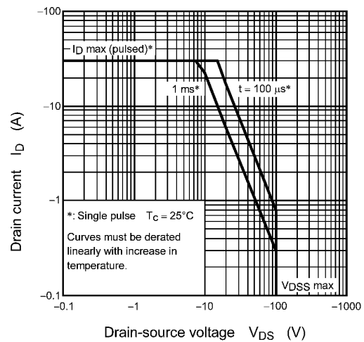
Fig. 8.13 Safe Operating Area (Guaranteed Maximum)
