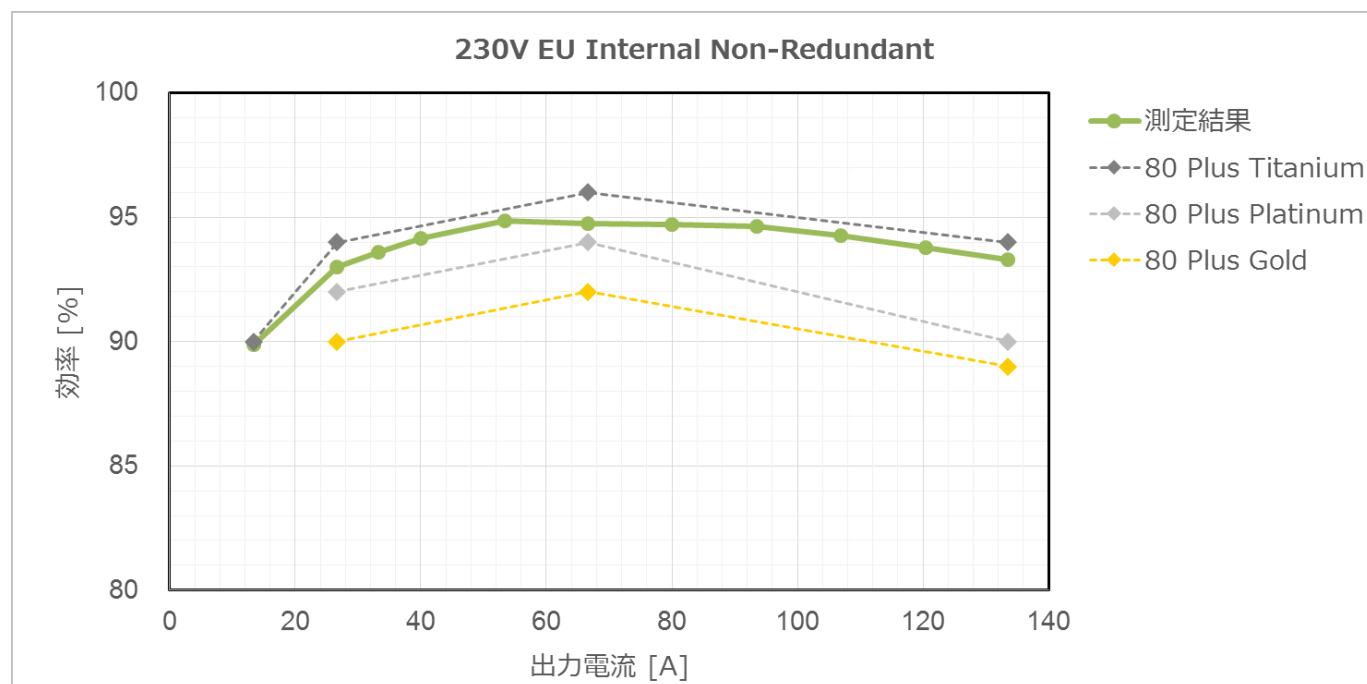
図 4.1.4 効率測定結果(80 PLUS:230V EU Internal Non-Redundant)
