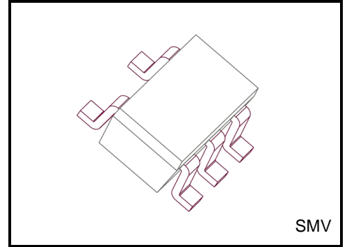
Weight: SMV (SOT-25) (SC-74A) : 16 mg (Typ.)
