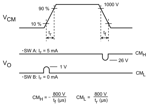
Fig. 13.1.8 Common-Mode Transient Immunity Test Circuit and Waveform
