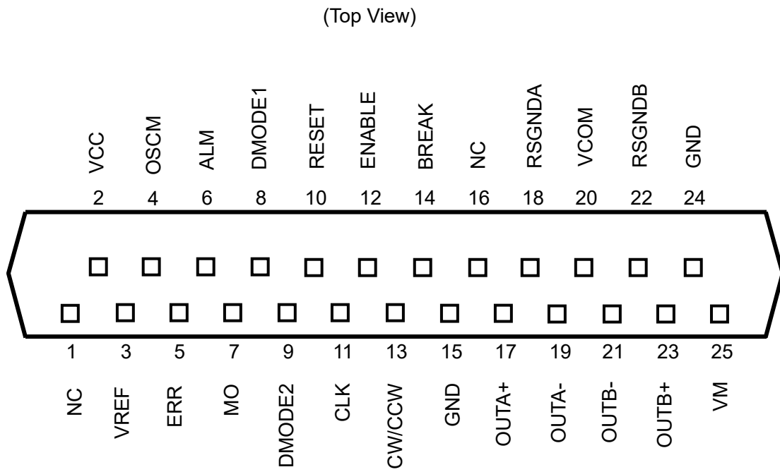
Figure 4.1 Pin Assignments (top view)
