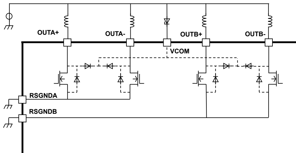
Figure 6.1 Break mode equivalent circuit
