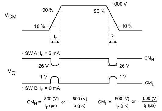
Fig. 13.1.8 Common-Mode Transient Immunity Test Circuit and Waveform
