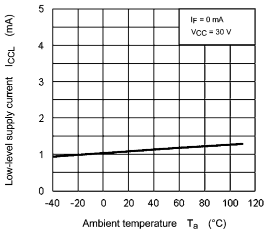
Fig. 13.2.5 I_{CCL} - T_a
