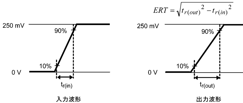
図 11.2 ERT (Equivalent Rise Time)
