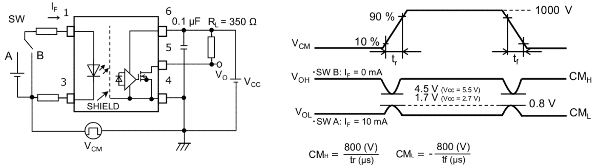
Fig. 12.1.7 Common-Mode Transient Immunity Test Circuit and Waveform
