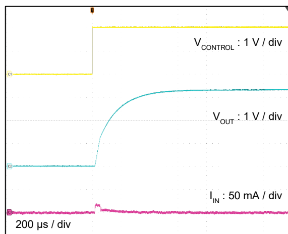
V_{OUT} = 3.3 V ( V_{IN} = 24.0 V )
