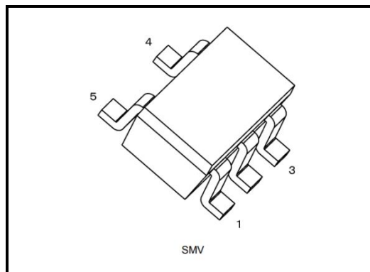
SMV (SOT-25) (SC-74A) Weight: 16 mg (Typ.)
