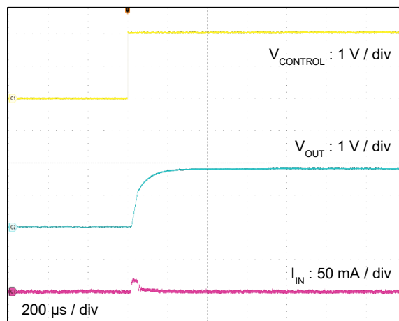
V_{OUT} = 1.8 V ( V_{IN} = 24.0 V )
