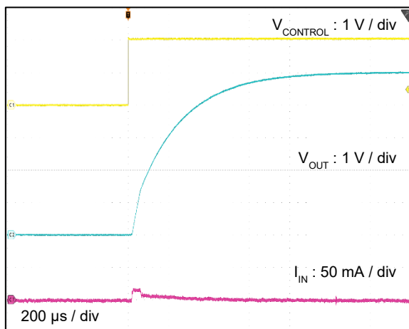
V_{OUT} = 5.0 V ( V_{IN} = 6.0 V )
