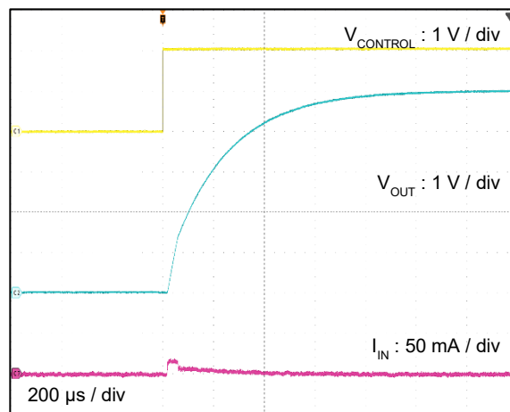
V_{OUT} = 5.0 V ( V_{IN} = 24.0 V )
