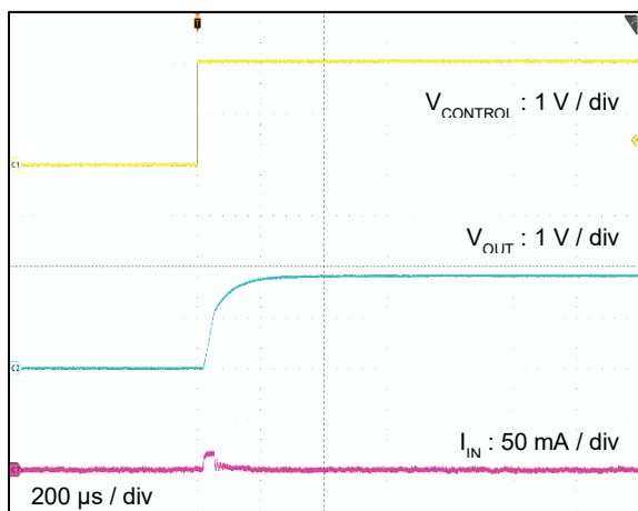
V_{OUT} = 1.8 V ( V_{IN} = 4.0 V )
