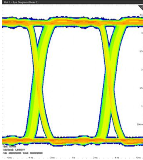
Fig. 14.1:DCL541L01 Eye diagram at 150Mbps
