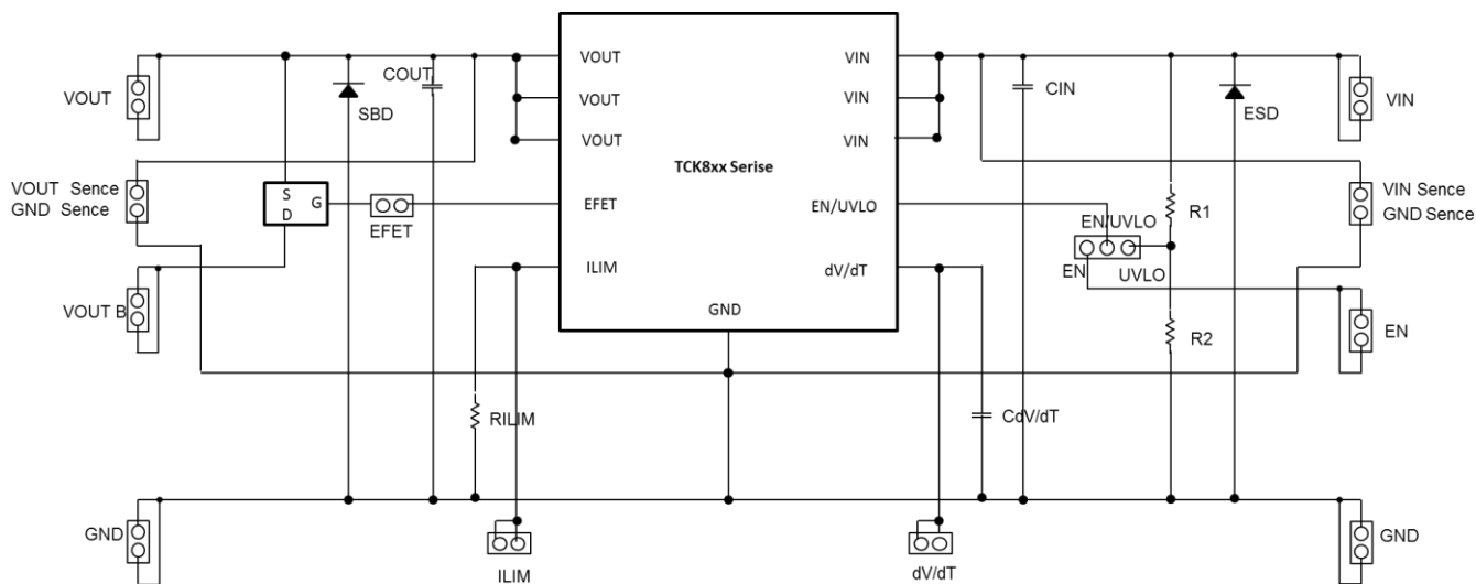
Figure 2-1 TCKE8xx EVB Schematic
