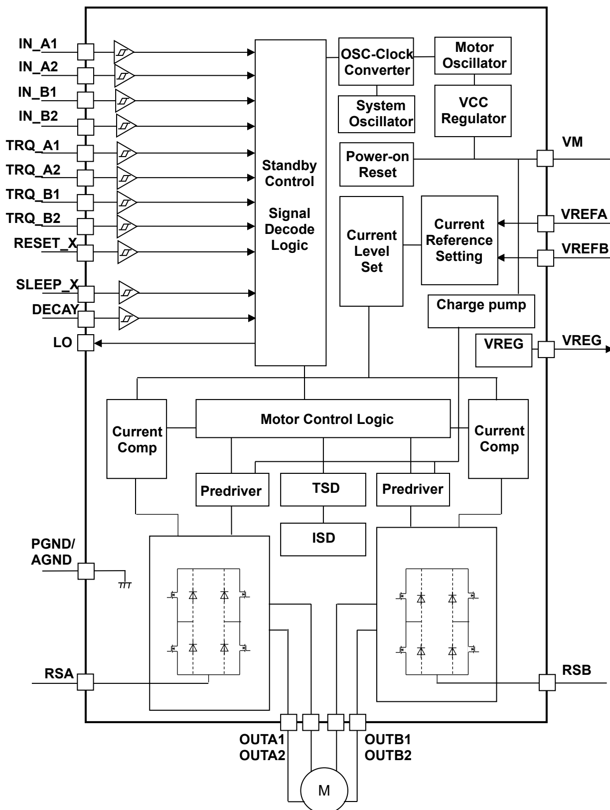
Fig. 4 Block diagram
