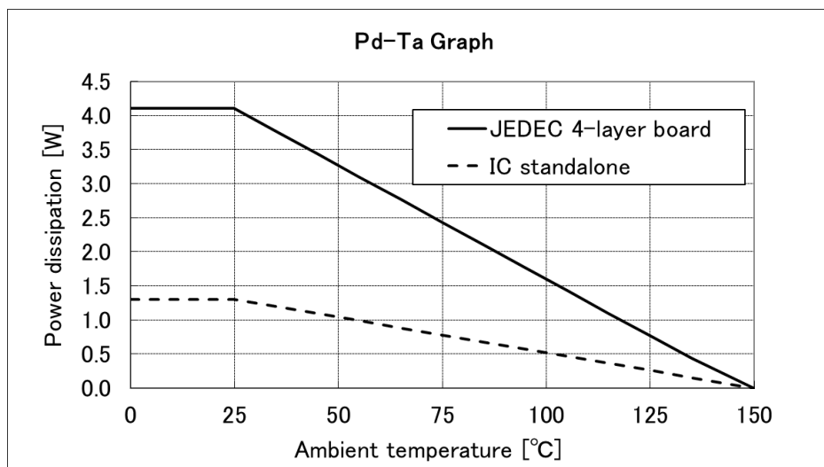
Figure13 PD-Ta graph
