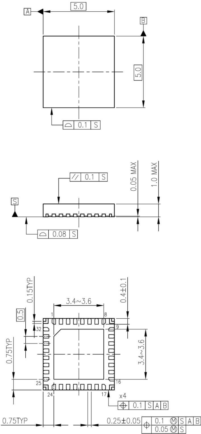
Figure17 Package Dimensions
