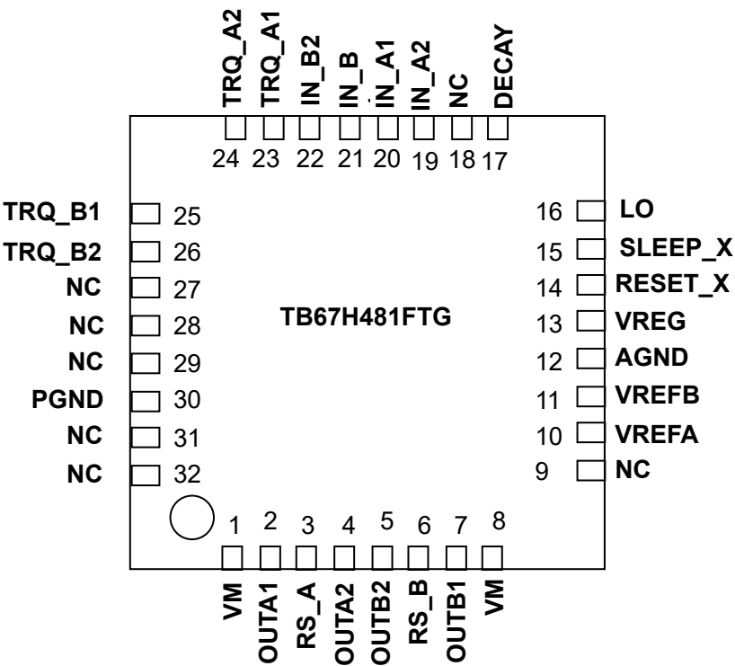
Figure3 Pin Assignment
