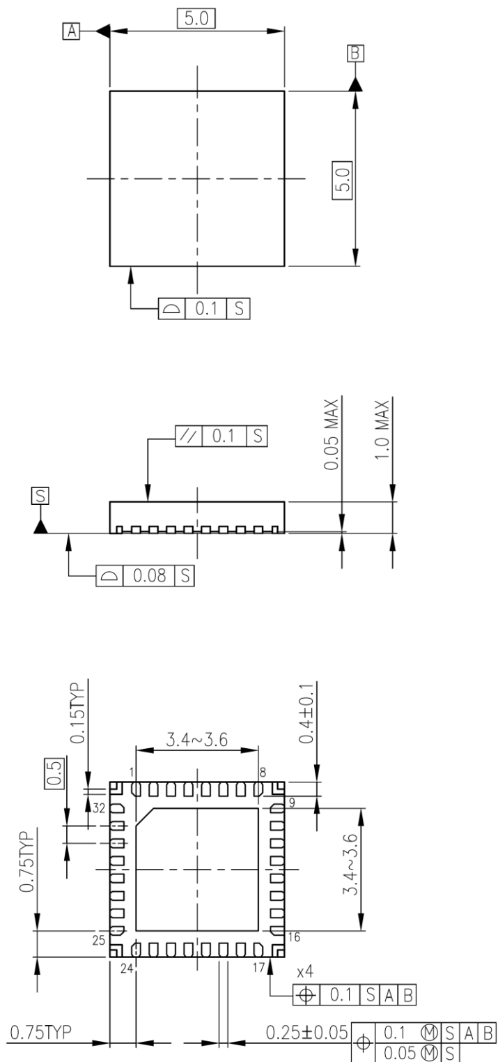
Figure 22 Package Dimensions
