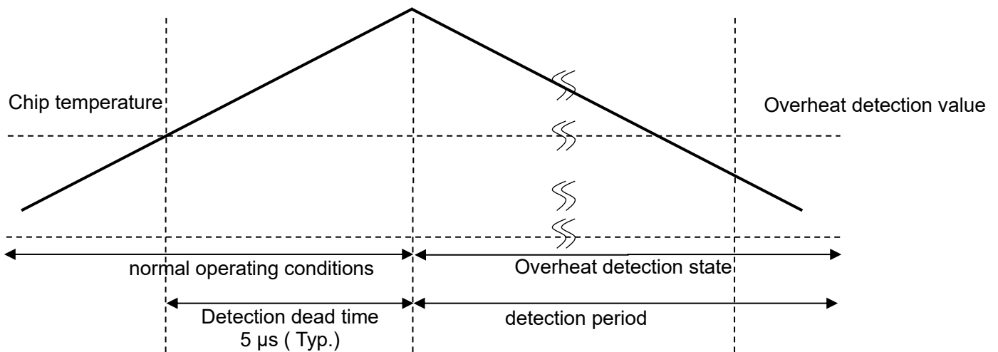
Figure 13 Overheat Detection
