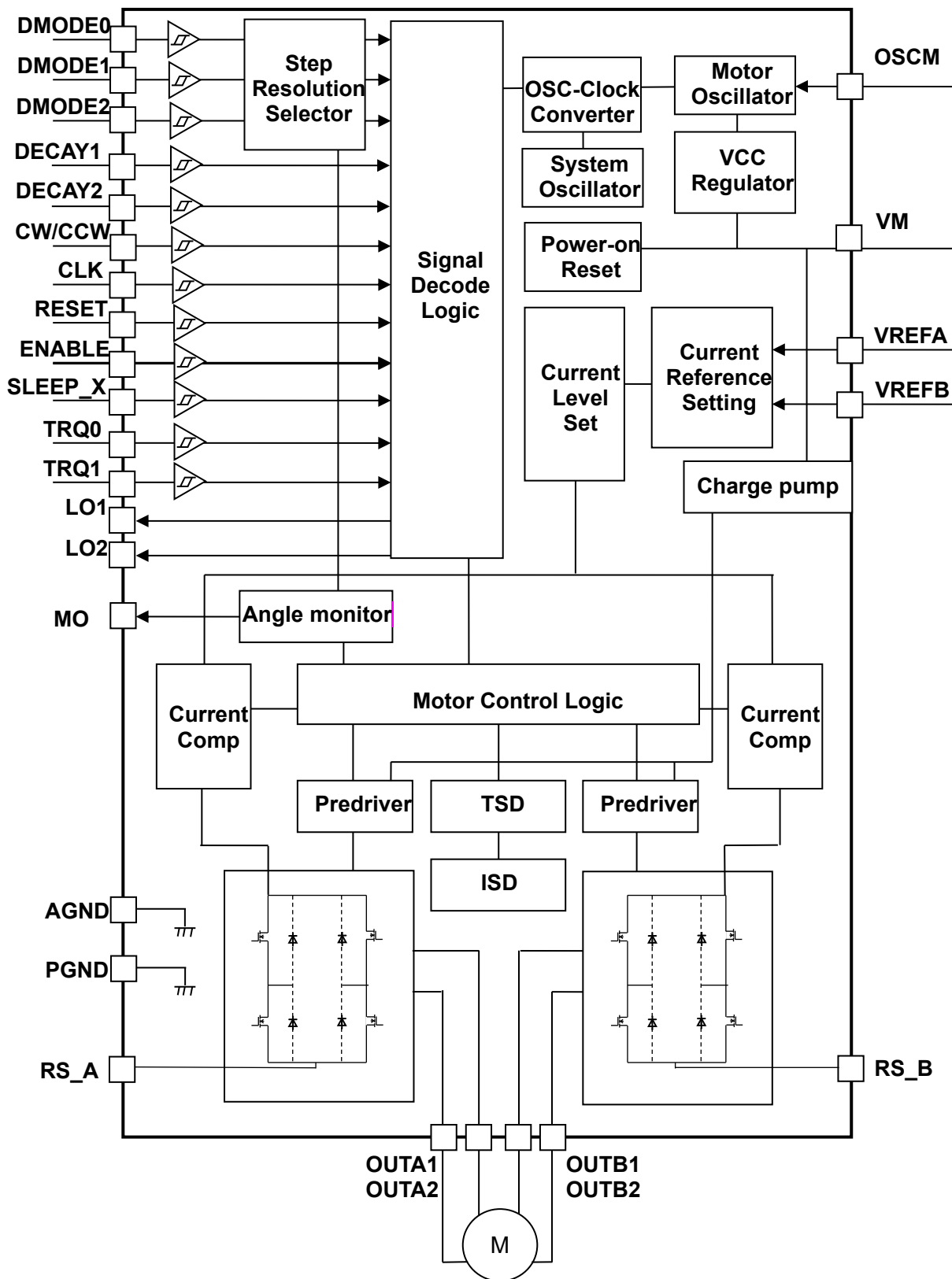
Figure 4 Block diagram
