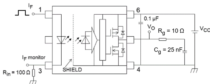
Fig. 13.1.7 Switching Time Test Circuit and Waveform
