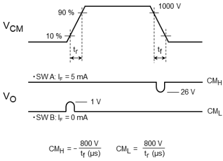
Fig. 13.1.8 Common-Mode Transient Immunity Test Circuit and Waveform
