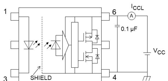
Fig. 13.1.6 I_{CCL} Test Circuit
