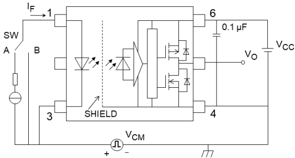
Fig. 13.1.8 Common-Mode Transient Immunity Test Circuit and Waveform
