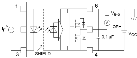
Fig. 13.1.1 I_{OPH} Test Circuit
