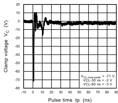
Fig. 10.4.6 ISO10605 Clamp Waveform -8 kV
