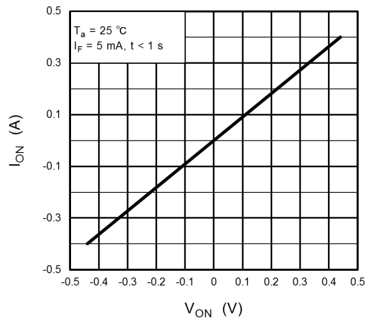
Fig. 12.4 I ON - V ON
