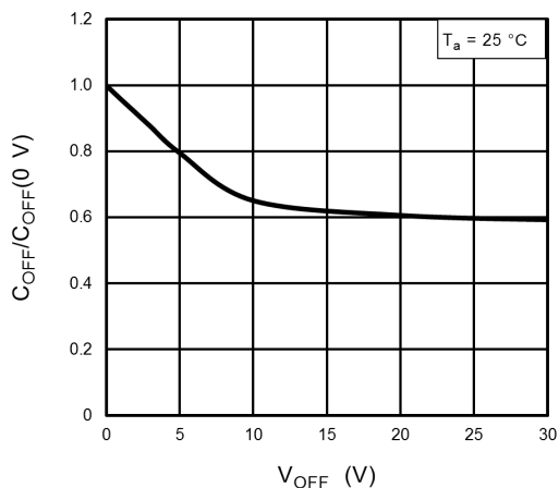
図 14.13 C_{OFF}/C_{OFF}(0V) - V_{OFF}
