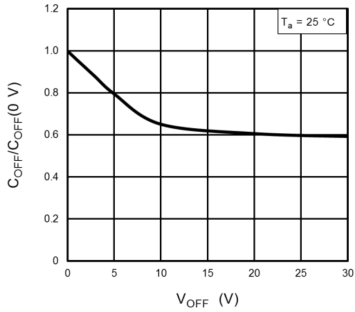
図 14.13 C_{OFF}/C_{OFF}(0V) - V_{OFF}
