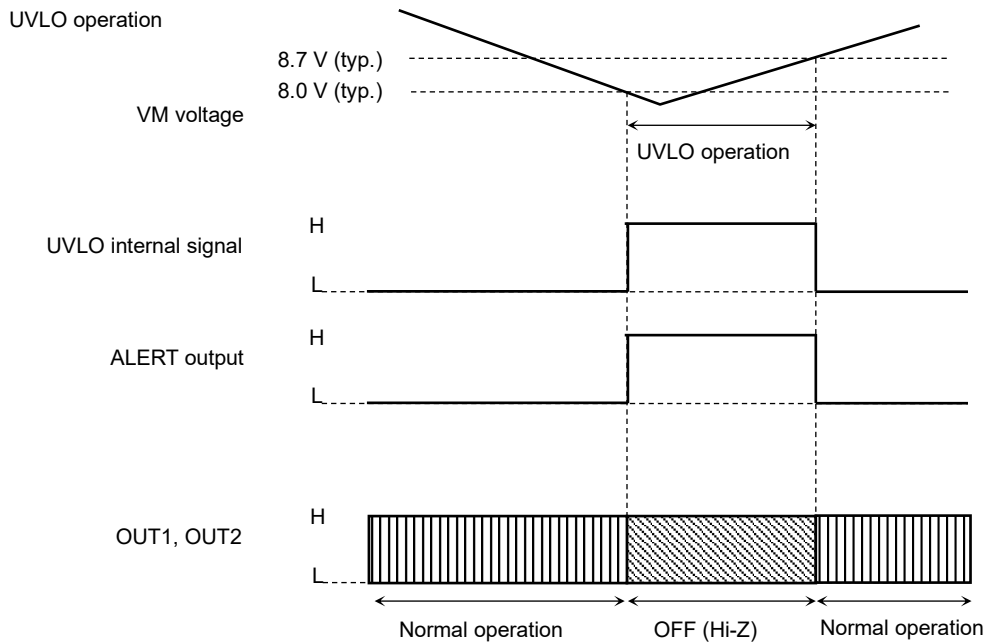
Figure 13.3 Timing Chart Example of UVLO Operation
