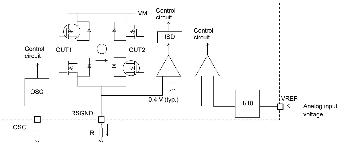
Figure 13.9.1 PWM Constant-current Control Circuit
