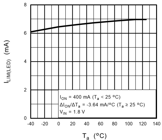
Fig. 12.12 I_{LIM(LED)} - T_a
