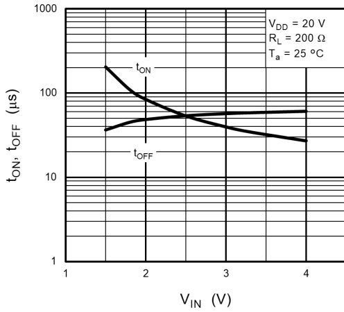
Fig. 12.7 t_{ON}, t_{OFF} - V_{IN}
