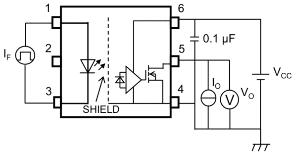
Fig. 13.1.5 IFHL, IFLH, IHYS Test Circuit
