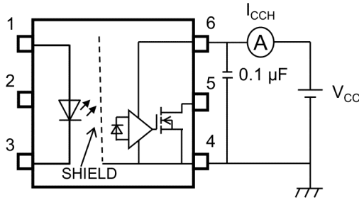
Fig. 13.1.3 ICCH Test Circuit
