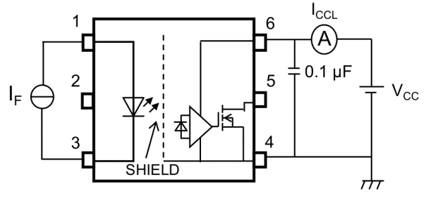
Fig. 13.1.4 ICCL Test Circuit
