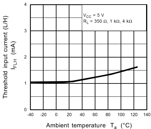
Fig. 13.2.9 I_{FLH} - T_a
