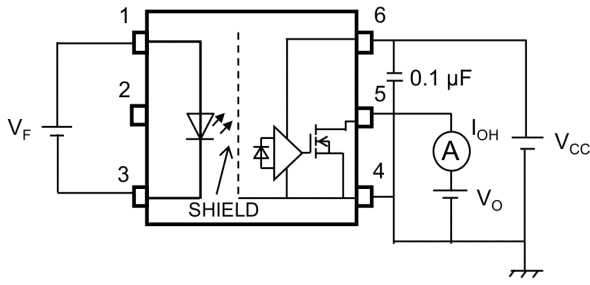
Fig. 13.1.1 IOH Test Circuit
