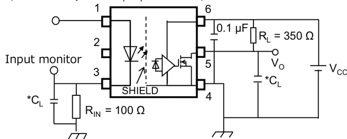
Fig. 13.1.6 Switching Time Test Circuit and Waveform
