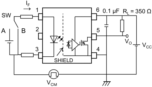
Fig. 13.1.7 Common-Mode Transient Immunity and Waveform
