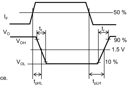
Fig. 13.1.6 Switching Time Test Circuit and Waveform
