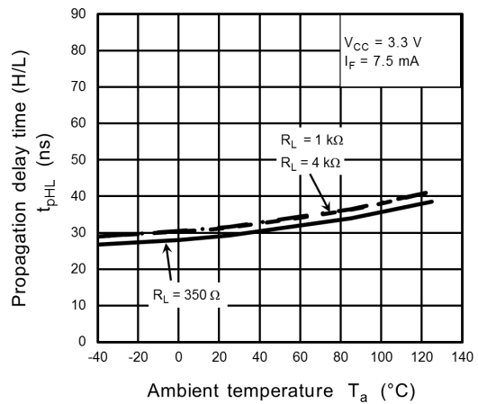
Fig. 13.2.16 t_{pHL} - T_a
