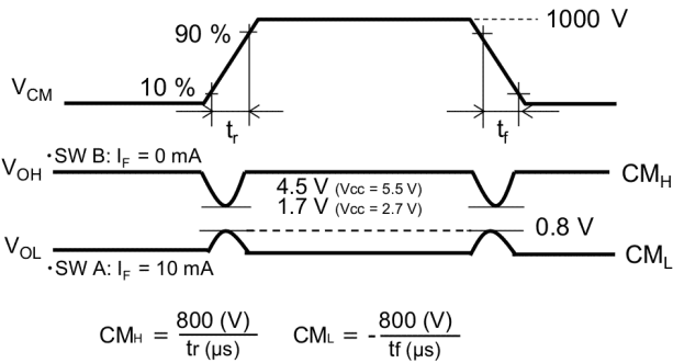
Fig. 13.1.7 Common-Mode Transient Immunity and Waveform
