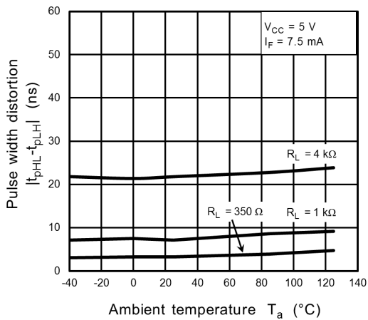
Fig. 13.2.15 |t_{pHL} - t_{pLH}| - T_a
