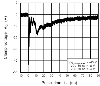
Fig. 10.7.4 IEC61000-4-2 Clamp Waveform -8 kV
