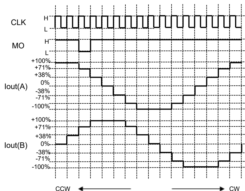
Figure 6.4 Half step resolution (Type B)
