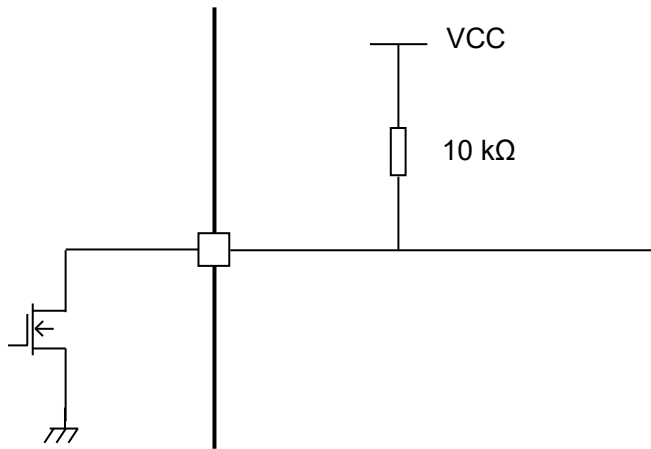
Figure 6.8 LO output pin
