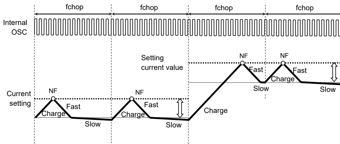
Figure 6.11 When the next current step is higher
