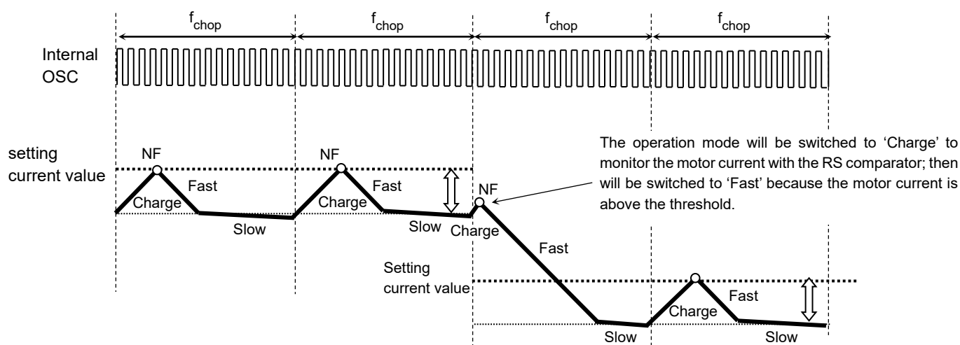
Figure 6.13 When the next current step is lower
