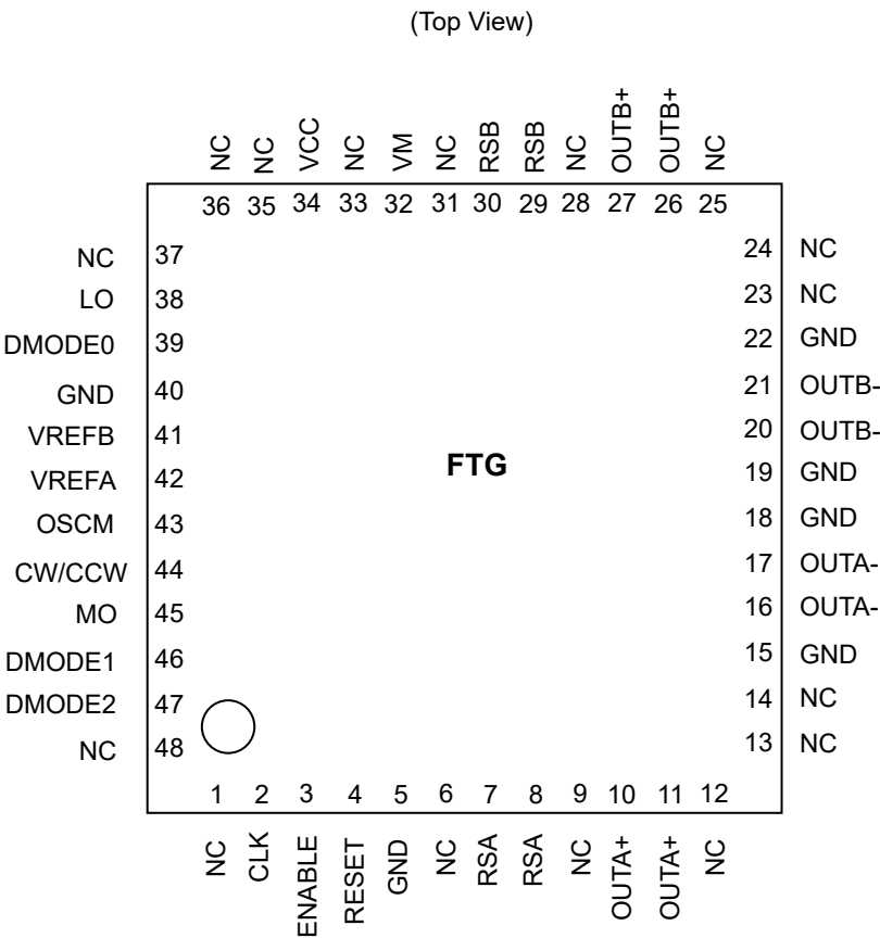
Figure 4.1 Pin Assignments
