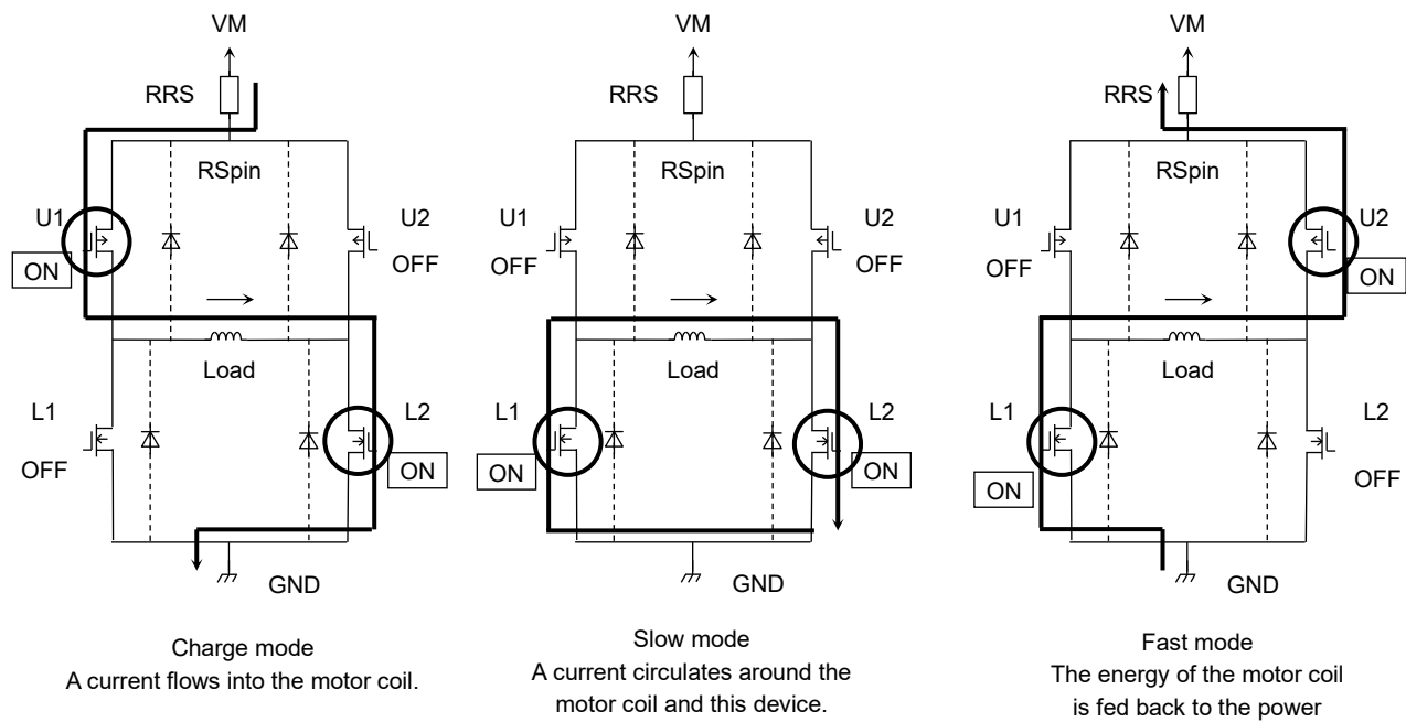
Figure 6.15 Output transistor function mode
