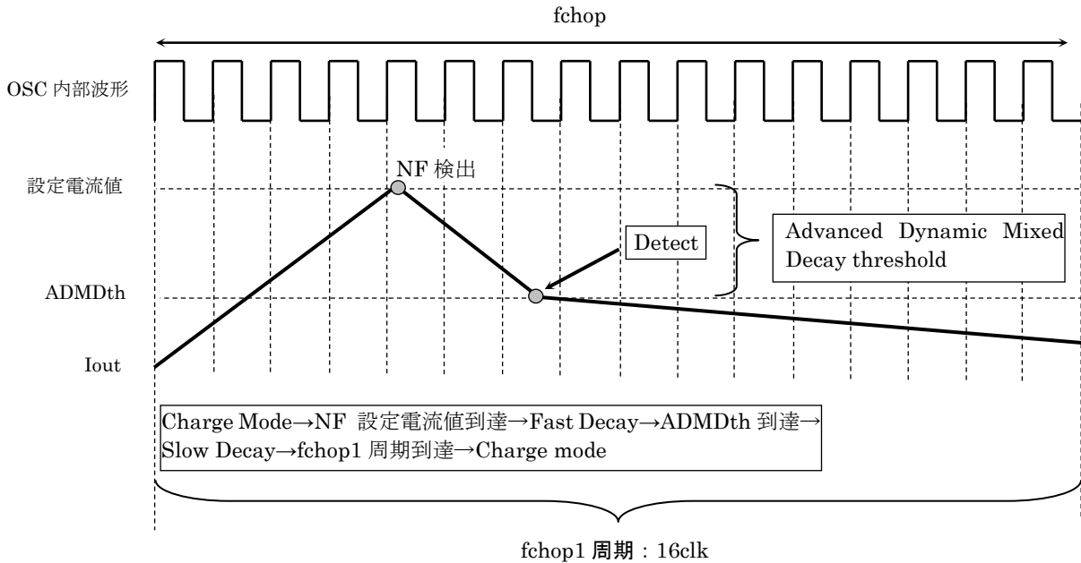
図 6.9 ADMD(Advanced Dynamic Mixed Decay)定電流制御
