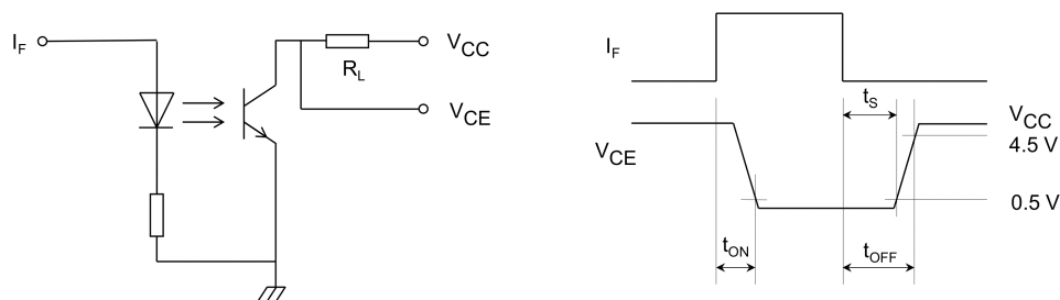
Fig. 11.1 Switching Time Test Circuit and Waveform
