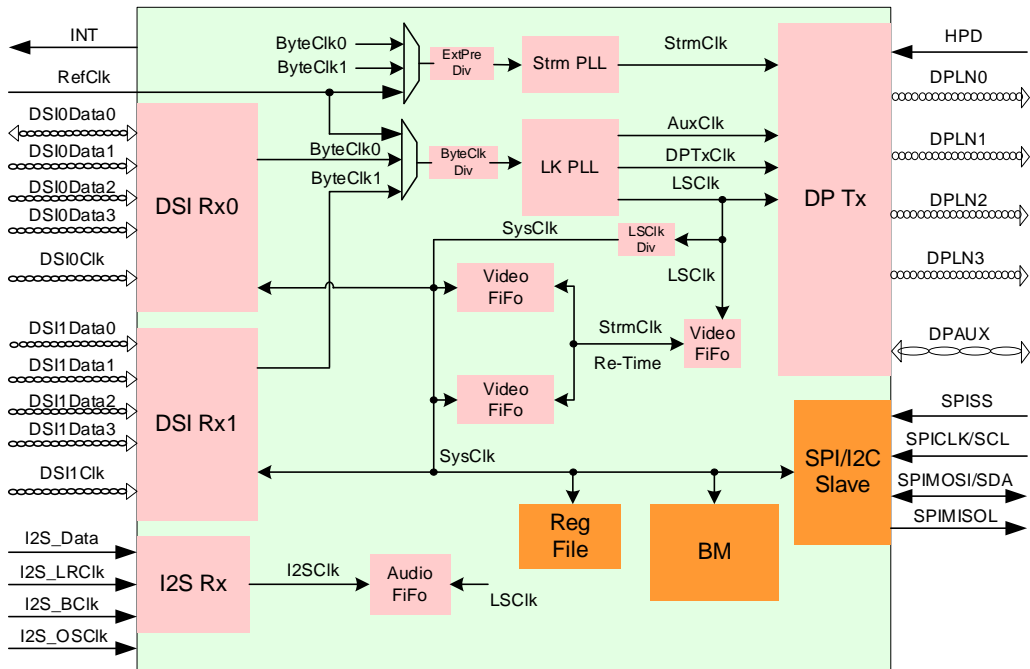
Figure 1.2 TC358770AXBG / TC358777XBG Block Diagram and Functional
