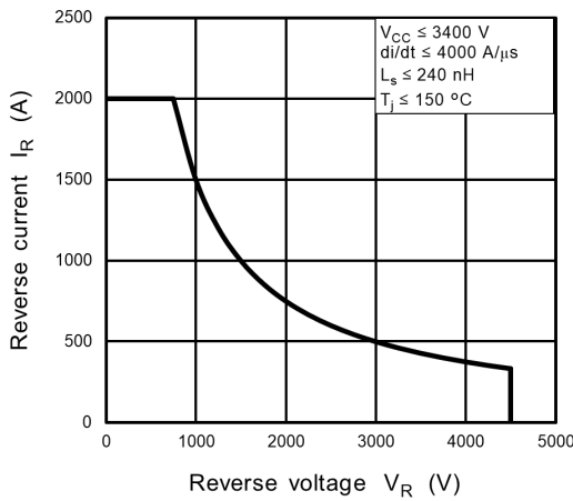
Fig. 7.15 RRSOA (Guaranteed value)
