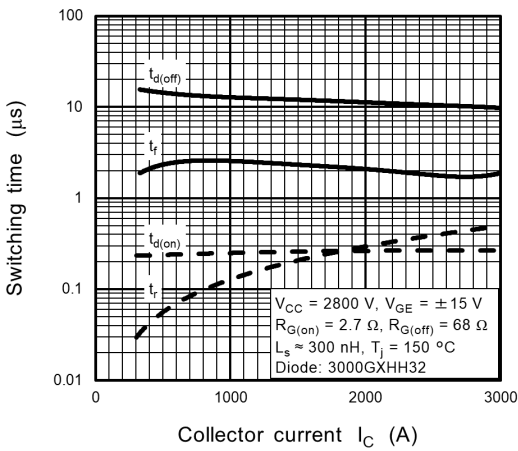
Fig. 7.9 Switching time - I_C
