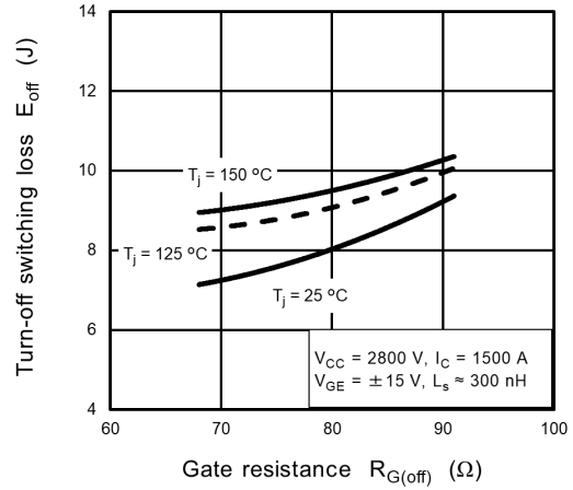
Fig. 7.8 E_{off} - R_{G(off)}
