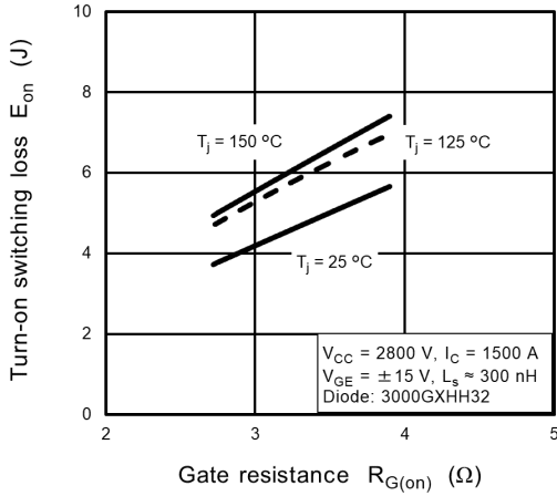
Fig. 7.7 E_{on} - R_{G(on)}
