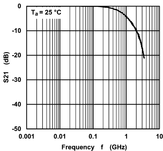
図 9.1 S_{21} - f
