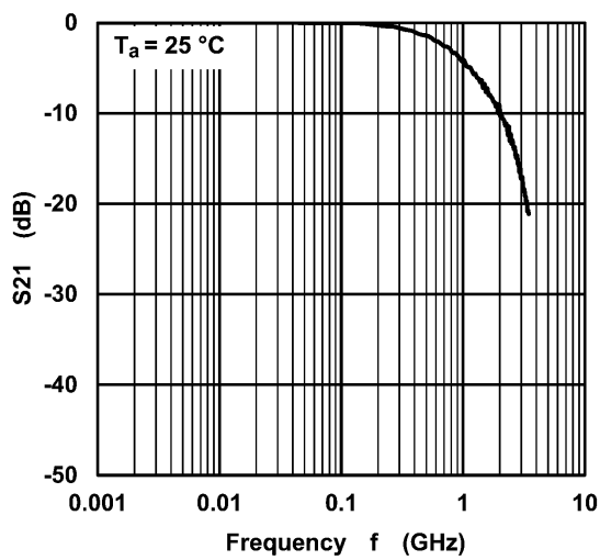
図 9.1 S_{21} - f
