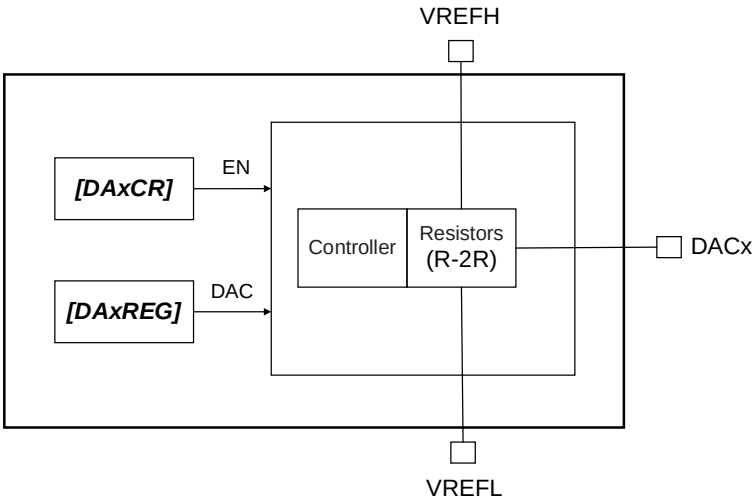
Figure 2.1 8-bit Digital to Analog Converter Configuration
