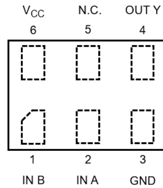
Pin Assignment
