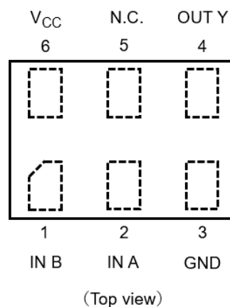
Pin Assignment
