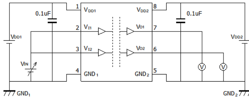
Fig. 12.3.1 DCL520C00/DCL520D00 V_{IH}/V_{IL} Test Circuit
