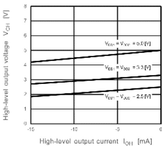
Fig.13.5 VOH-IOH
