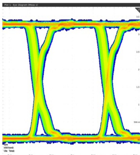
Fig.14.1 DCL521xx00 Eye diagram at 150Mbps
