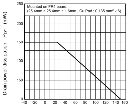
Fig. 7.11 P_{D^*} - T_a
