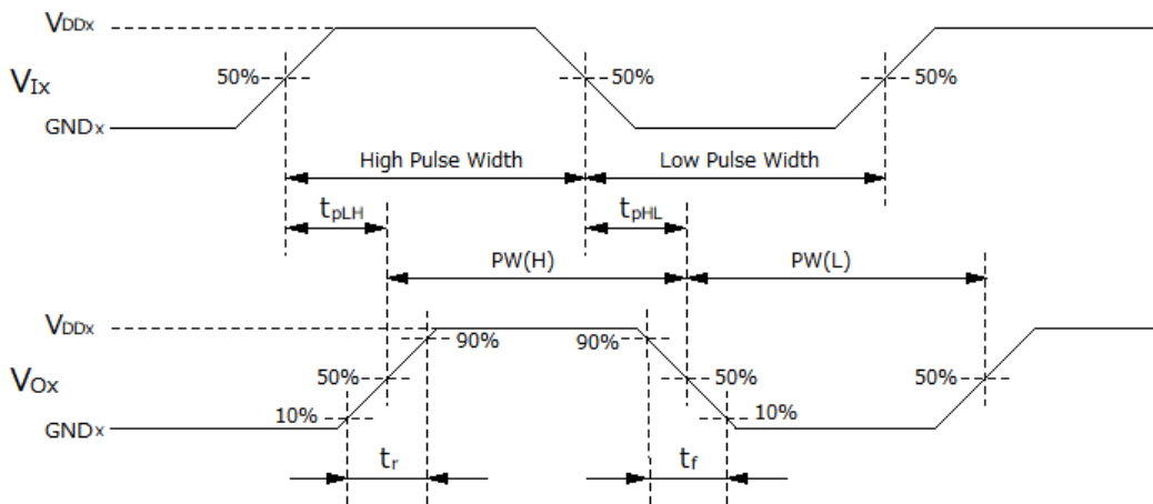
Figure12.4 Switching Waveforms
