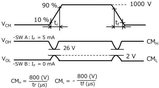
Fig. 13.1.7 Common-Mode Transient Immunity Test Circuit and Waveform
