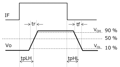
Fig. 13.1.6 Switching Time Test Circuit and Waveform
