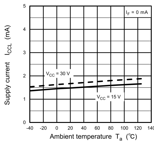
Fig. 13.2.5 I_{CCL} - T_a
