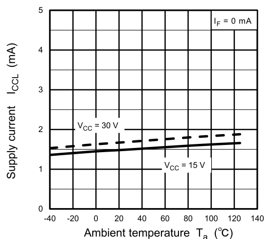
Fig. 13.2.5 I_{CCL} - T_a
