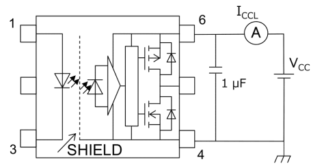
Fig. 13.1.5 I_{CCL} Test Circuit
