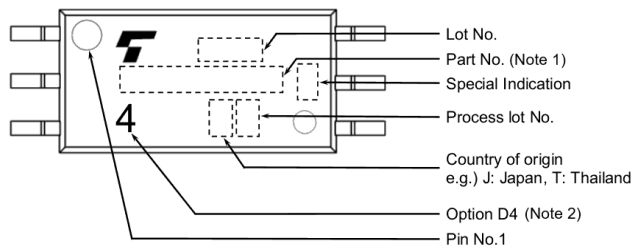
Fig. 17.3 Marking Example
