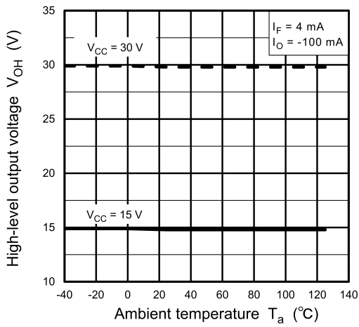
Fig. 13.2.9 V_{OH} - T_a
