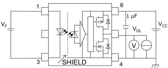
Fig. 13.1.3 V_{OL} Test Circuit
