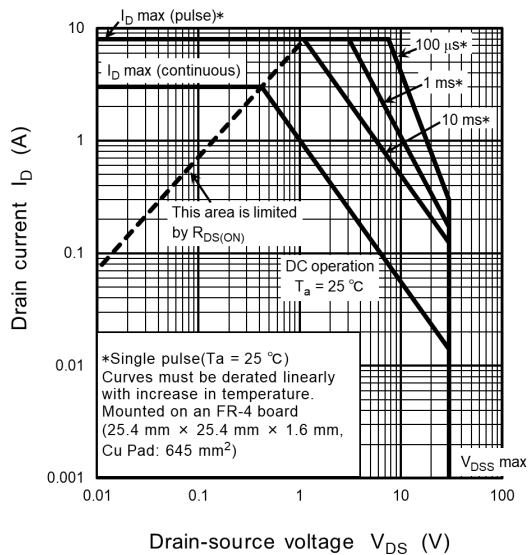
Fig. 9.11 Safe Operating Area
