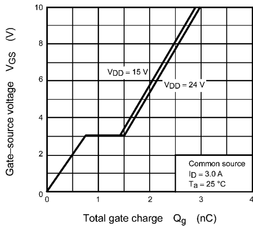
Fig. 7.9 Dynamic Input/Output Characteristics
