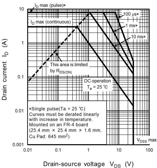
Fig. 7.11 Safe Operating Area
