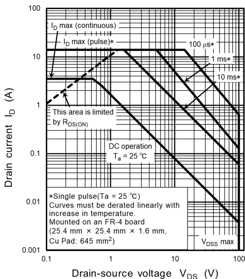
Fig. 7.10 Safe Operating Area
