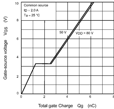
Fig. 7.8 Dynamic Input Characteristics
