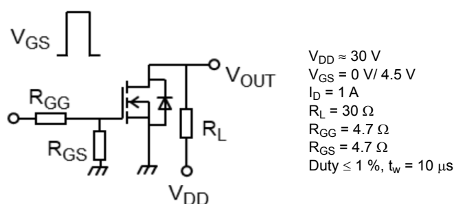
Fig. 5.2.1 Switching Time Test Circuit
