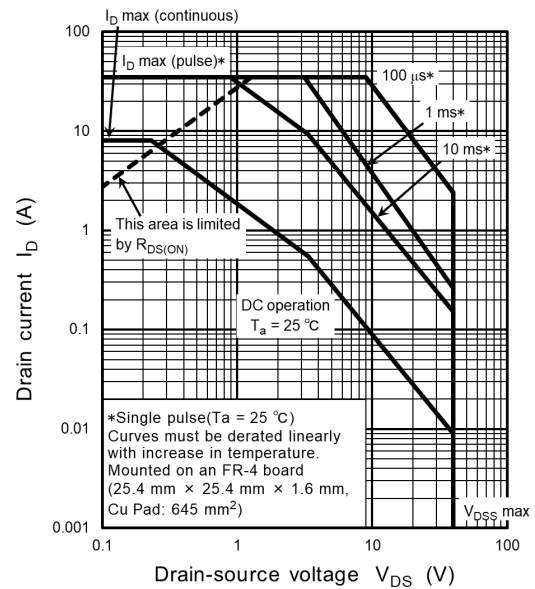
Fig. 9.10 Safe Operating Area
