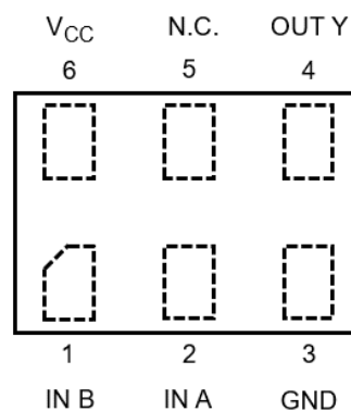
Pin Assignment
