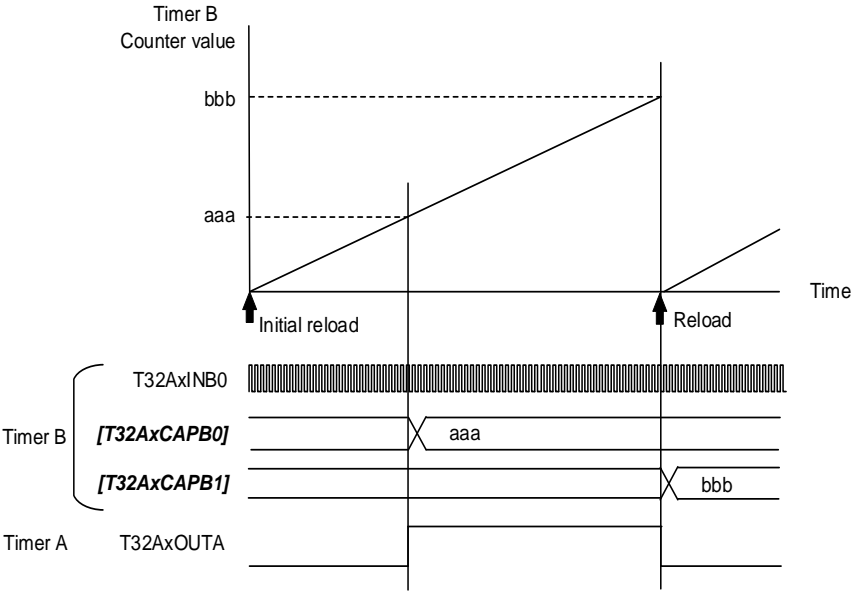
Figure 5.9 Frequency Measurement Using Capture Function
