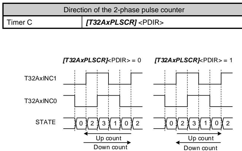
Figure 3.1 State Transition
