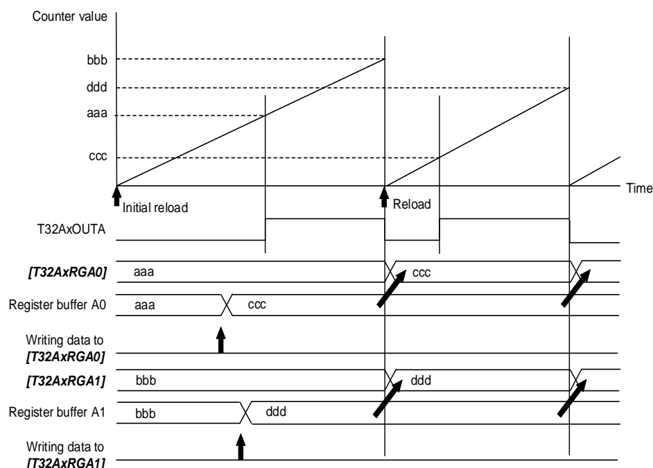
Figure 5.4 Example of PPG Output (Low Active)
