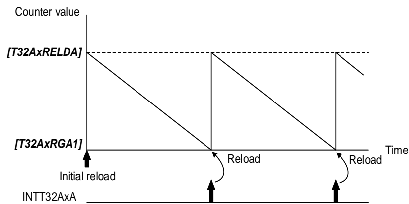
Figure 5.2 Interval Timer (Count Down)
