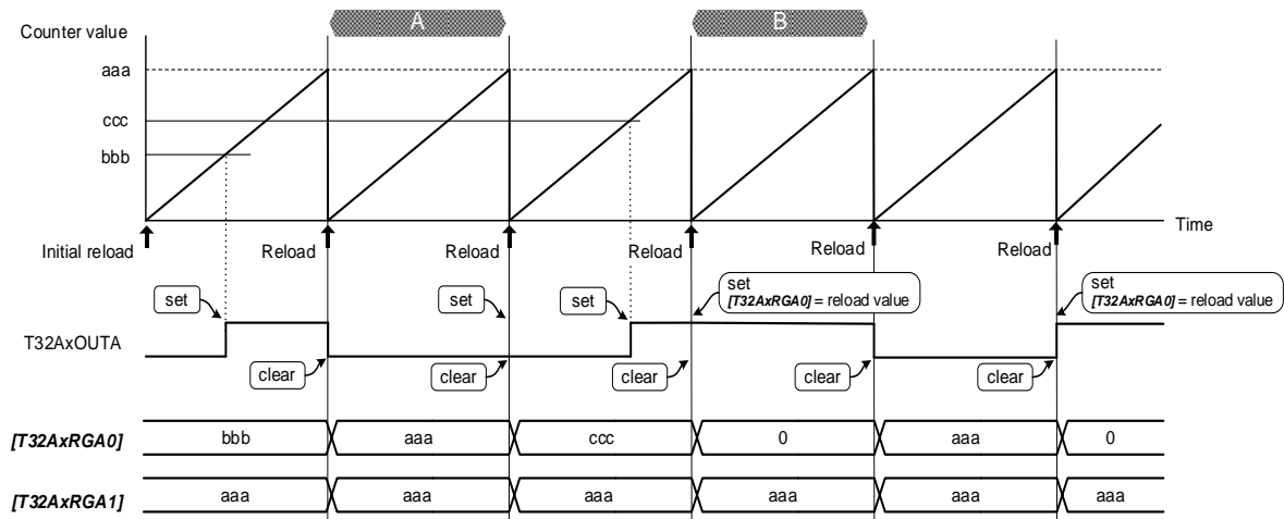
Figure 5.5 PPG Output (<Period A, B>)
