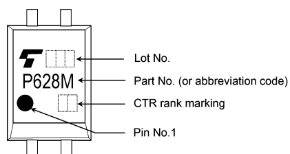
Fig. 14.1 Marking example of TLP628M
