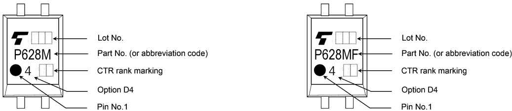
Fig. 15.4 Marking Example of TLP628M (Note 1) Fig. 15.5 Marking Example TLP628MF (Note 1)
