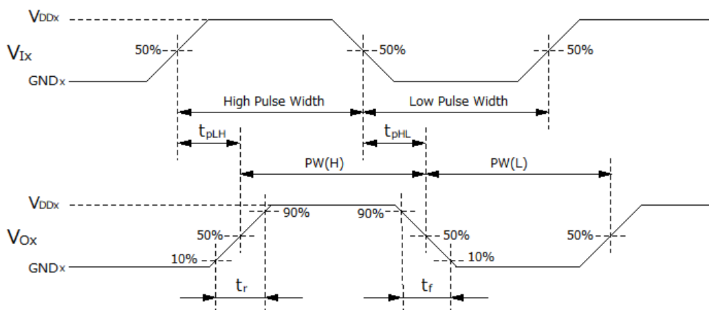
Fig.12.4.6. DCL5xx01A Switching characteristic waveform diagram
