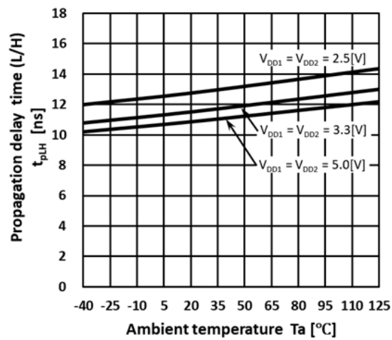
Fig.13.7. Propagation Delay Time t_{pLH} - T_a
