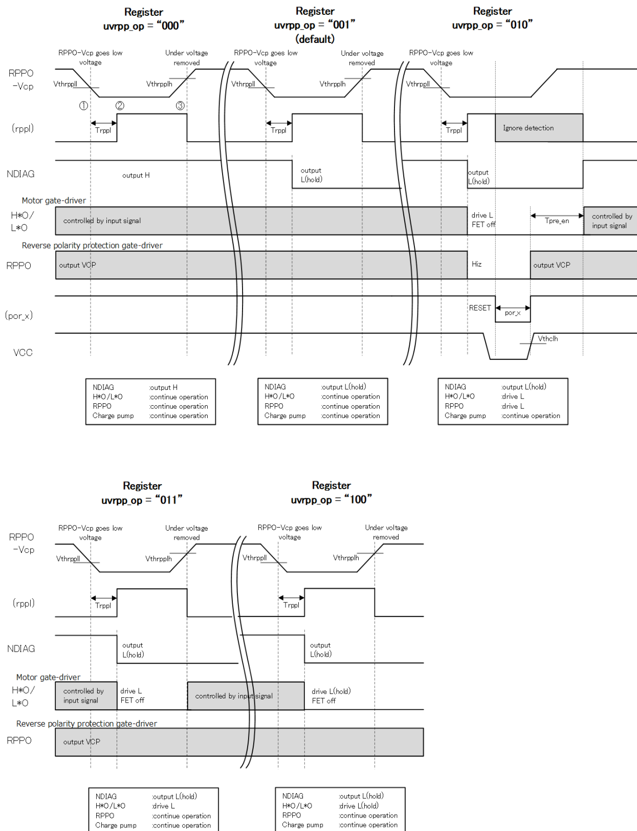
Fig. 7.6.3.2 RPPU Under Voltage Detection Timing Chart
