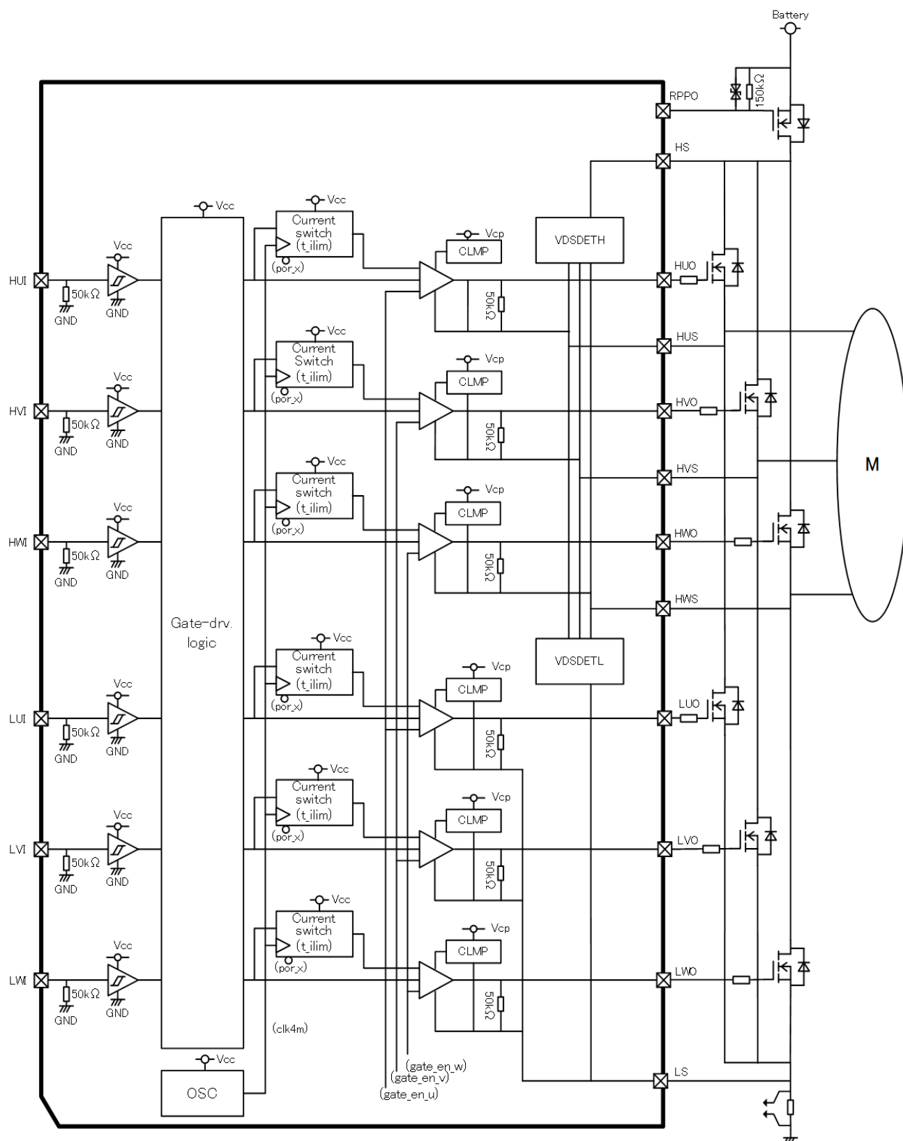
Fig. 7.2.1.1 Gate Driver Circuits Block Diagram
