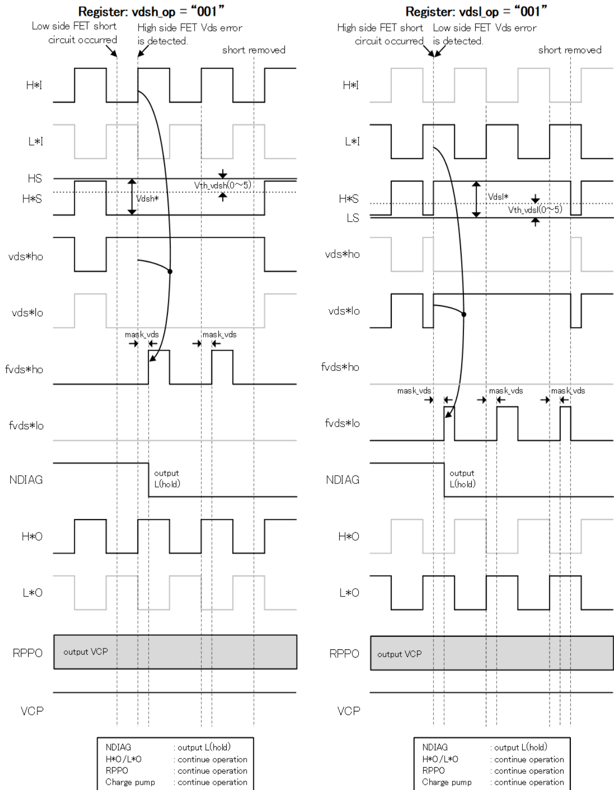
Fig. 7.6.7.3 Short-Circuit Detection Timing Chart (In the case of register: vds l _op = vds h _op "001")
