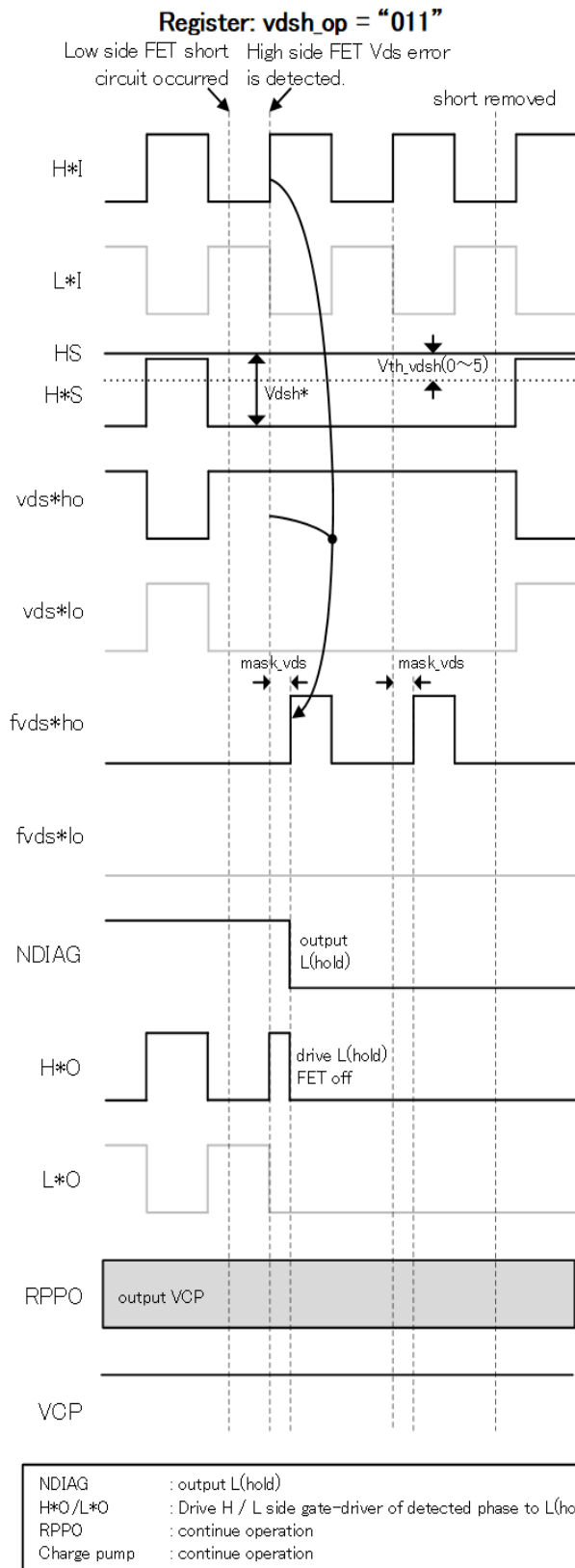
Fig. 7.6.7.5 Short-Circuit Detection Timing Chart (In the case of register: vds l _op = vds h _op "011")
