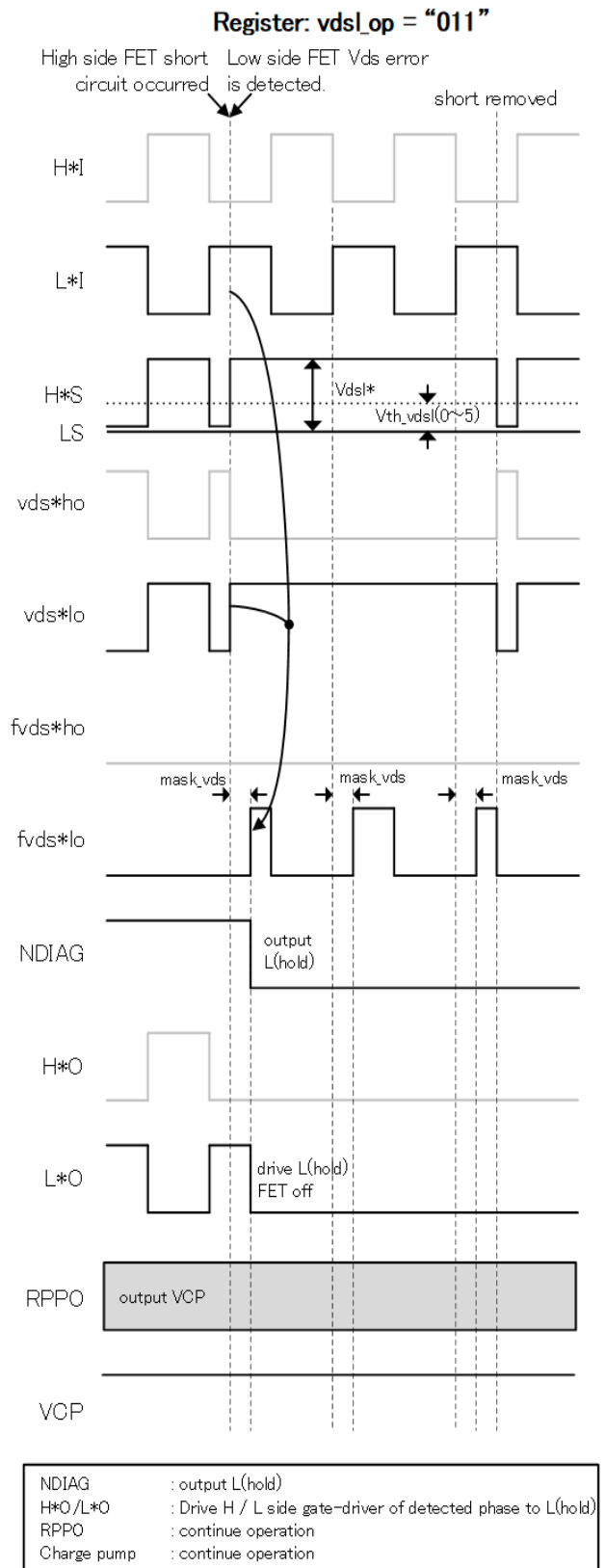
Fig. 7.6.7.5 Short-Circuit Detection Timing Chart (In the case of register: vds l _op = vds h _op "011")
