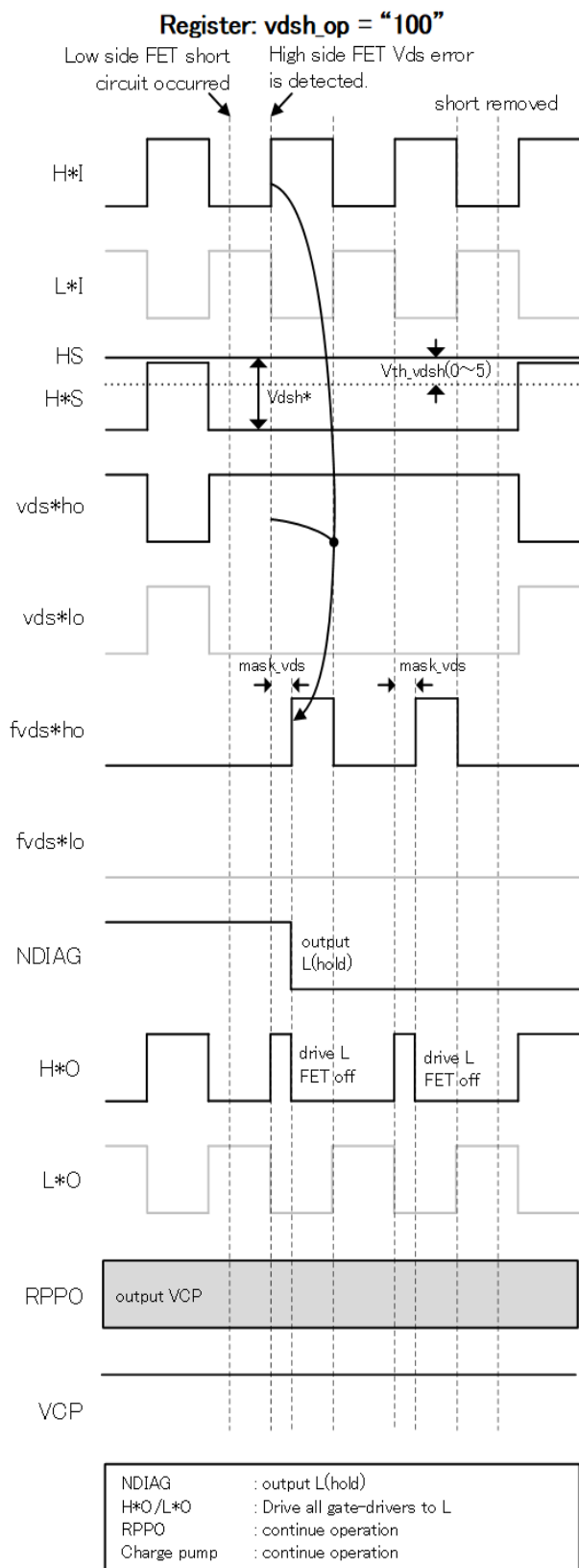
Fig. 7.6.7.6 Short-Circuit Detection Timing Chart (In the case of register: vds l _op = vds h _op "100")
