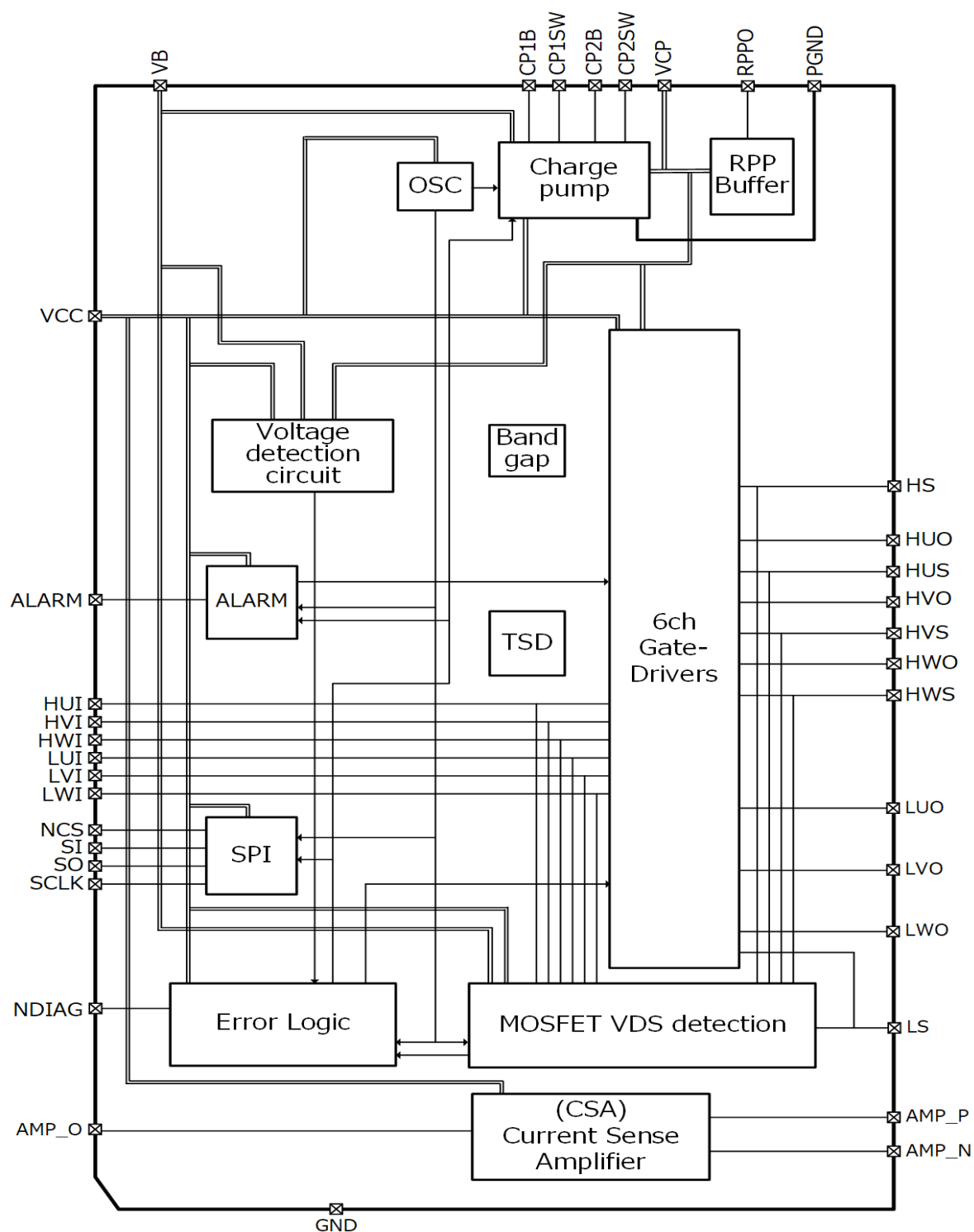
Fig. 4.1 Block Diagram
