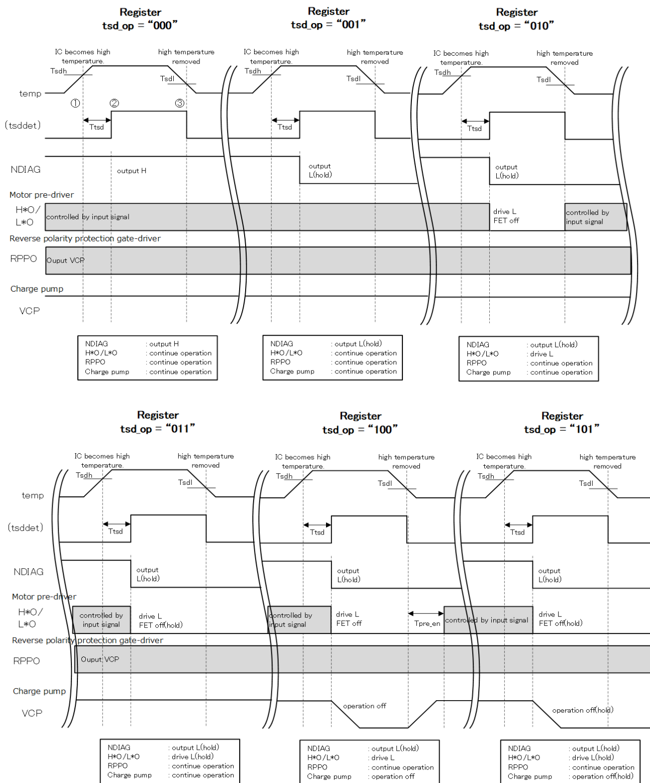
Fig. 7.6.6.2 Over Temperature Detection Timing Chart
