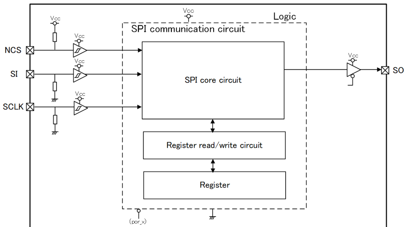
Fig. 7.8.1 SPI Communication Circuit Block Diagram
