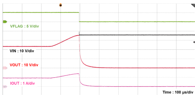
図 12.17 TCKE601RA 過電圧保護時の波形 V_{IN} = 24\text{ to }35\text{ V} , C_{OUT} = 1\text{ }\mu\text{F} , R_{ILIM} = 11\text{ k}\Omega , R_{OUT} = 25\text{ }\Omega
