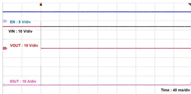
図 12.15 TCKE603RL 短絡保護時の波形 (ラッチタイプ) V_{IN} = 24\text{ V} , C_{OUT} = 1\text{ }\mu\text{F} , R_{ILIM} = 11\text{ k}\Omega , R_{OUT} = \text{Open to short}
