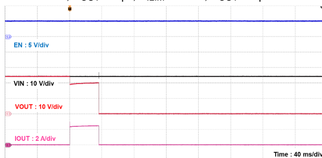
図 12.12 TCKE603RL 過電流保護時の波形 (ラッチ) V_{IN} = 24\text{ V} , C_{OUT} = 1\text{ }\mu\text{F} , R_{ILIM} = 11\text{ k}\Omega , R_{OUT} = \text{Open to } 8\text{ }\Omega
