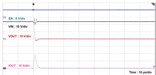
図 12.16 TCKE603RL 短絡保護時の波形 (拡大) V_{IN} = 24\text{ V} , C_{OUT} = 1\text{ }\mu\text{F} , R_{ILIM} = 11\text{ k}\Omega , R_{OUT} = \text{Open to short}
